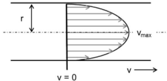
Abb. 1: The picture shows a liquid flöwing through a pipe with the simplifyfication of the fluid layers. r - is the capillaryradius and v is the flowspeed. [1]
